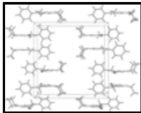
Fig. 2. Packing diagram of the title compound viewed along the c axis.
